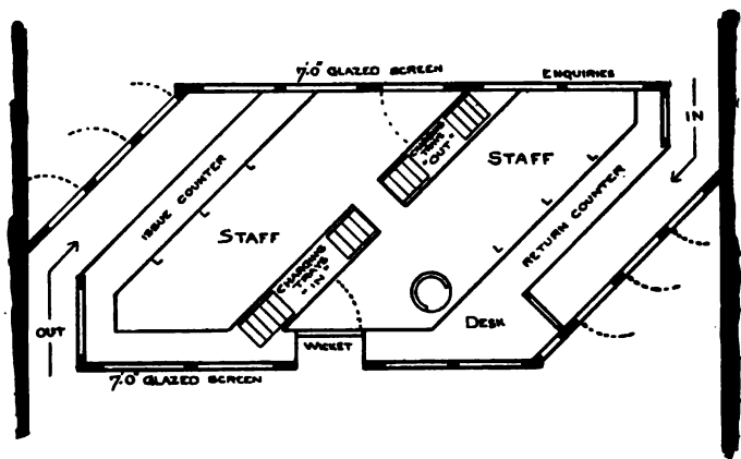
FIG. 26.—Plan of Triple Open-Access Barrier, Section (Section 160).
